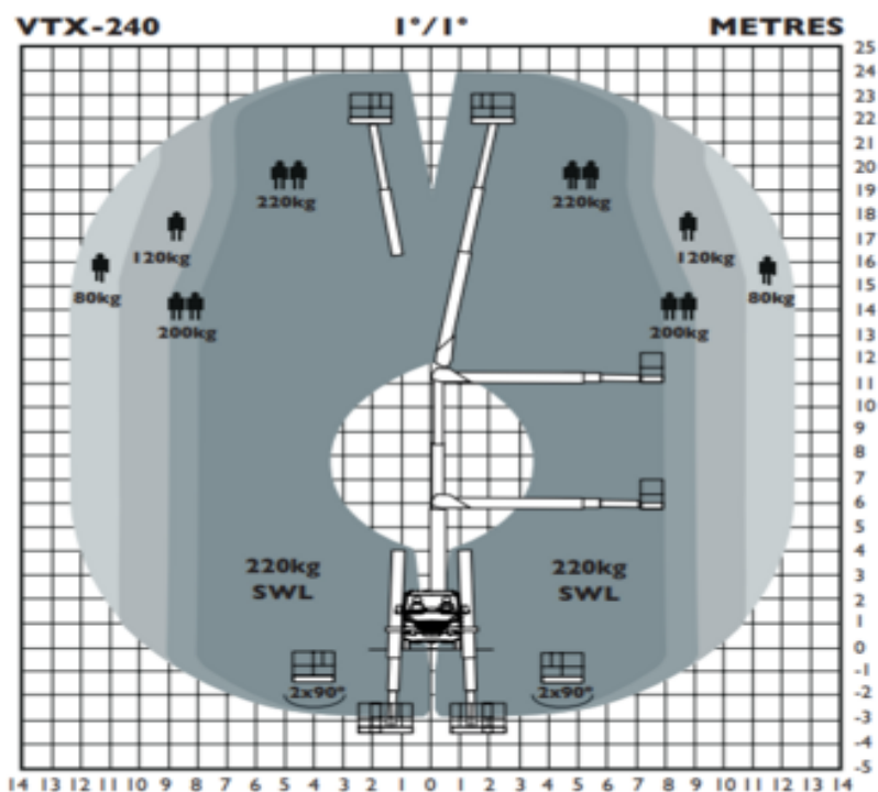
Working envelope at 80/120/200/220kg bucket SWL
