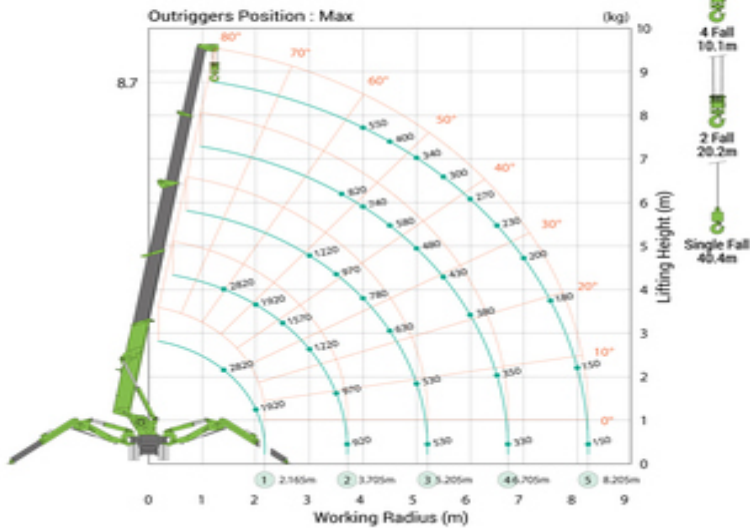
Working Range Chart (4 falls)
