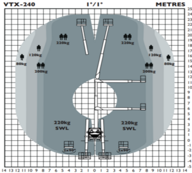
Working envelope at 80/120/200/220kg bucket SWL
